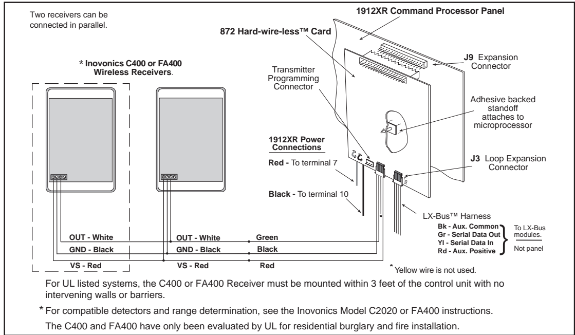
Figure 1: Wiring for the 400 series receiver(s) and 872 card.
